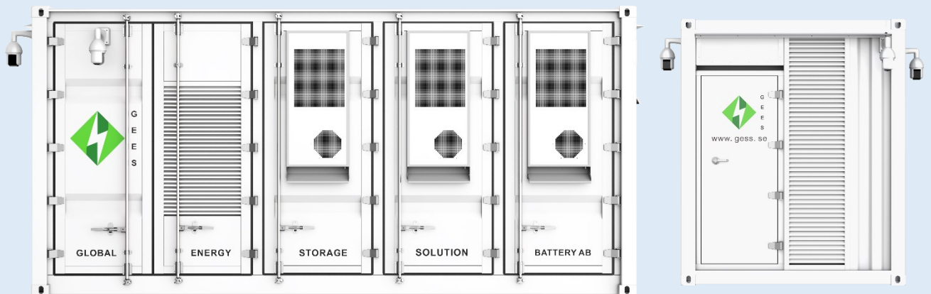
GESS-SW-1000TH-PO side views
