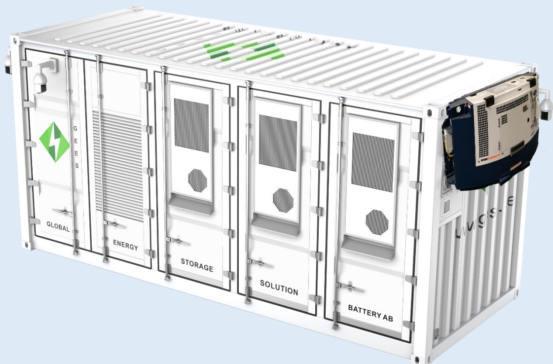
GESS-SW-825TH-PO with Clip-On Genset attached
